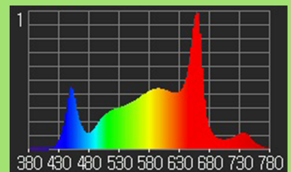
McCree Kurve (RQE)
